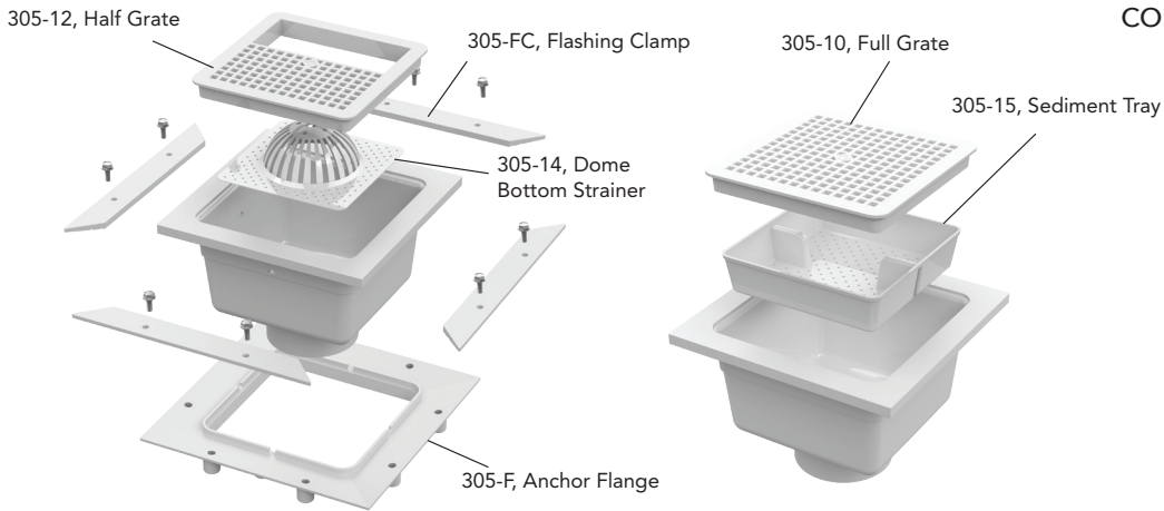
FIG. # 305 Shown with Dome Bottom Strainer
