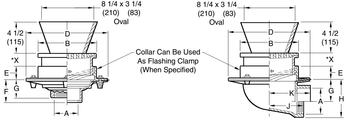
8 1/2"(215) 12"(305)... TOP SIZE = B DIA..... 8 1/2"(215) 12"(305) Fig. ... 3650C ... 3655C ..... CAULK OUTLET.... Fig. ... 3660C ... 3665C Fig. ... 3650T ... 3655T ... THREADED OUTLET... Fig. ... 3660T ... 3665T
