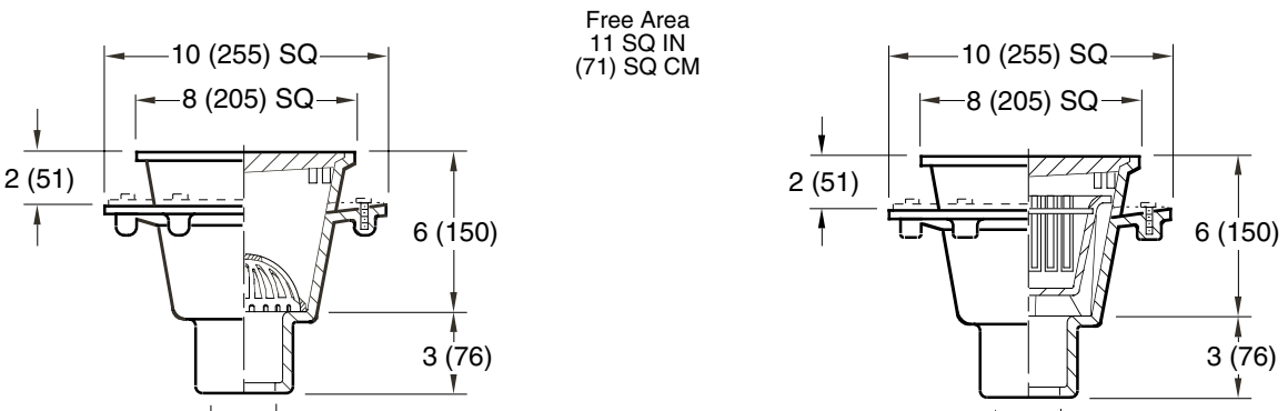
A (Pipe Size) = 02(50), 03(75) or 04(100) WITH DOME BOTTOM STRAINER WITH SEDIMENT BUCKET
