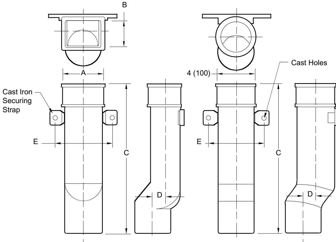
Fig. 1785 Series ... 4(100) x 3"(76) RECTANGULAR Fig. 1786 Series ... 5(125) x 4"(100) RECTANGULAR
