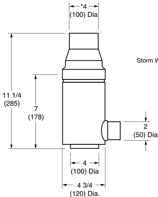
Fig. RH9508-04...4" OUTLET * Sized to accept Downspout Converter and 4" S & D Pipe
