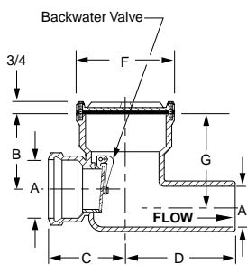
Fig. 7012 Bolted Cover
