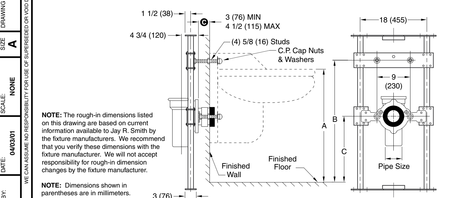
Fig. 0925 . . . WITH SUPPORTING STUDS, ADJUSTABLE COUPLING AND WASTE FITTING 4" (100) CAULK AND 4" (100) VENT FOR BACK OUTLET FLUSHING RIM SERVICE SINK
