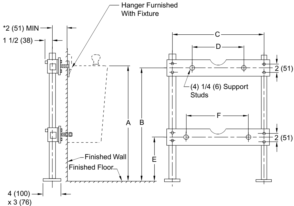
Fig. 0830 . . . FOR WALL MOUNTED ELECTRIC WATER COOLERS
