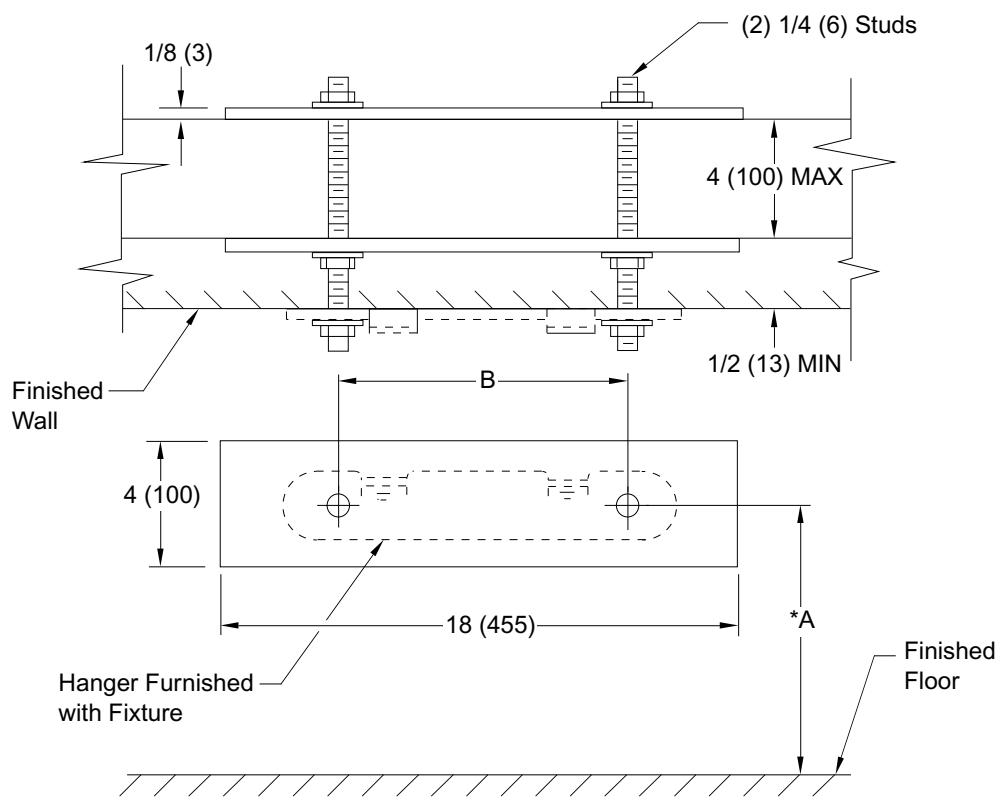
Fig. 0825 . . . DOUBLE REINFORCING PLATES FOR HIGH BACK LAVATORIES WITH CONCEALED HANGER
