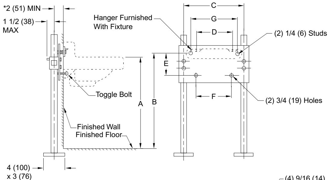
Fig. 0805... WITH PLATE AND STUDS FOR HIGH BACK LAVATORIES WITH CONCEALED WALL HANGER AND EXTENDED BOTTOM SECURING LUGS
