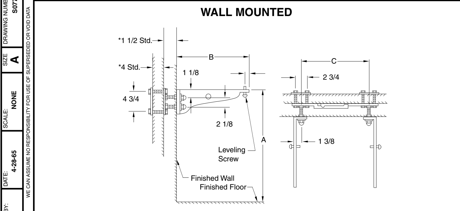
Fig. 0772 . . . WITH OFFSET ACID RESISTANT COATED EXPOSED ARMS FOR HIGH BACK ENAMELED IRON LAVATORIES SET ON MASONRY OR STUD WALL
