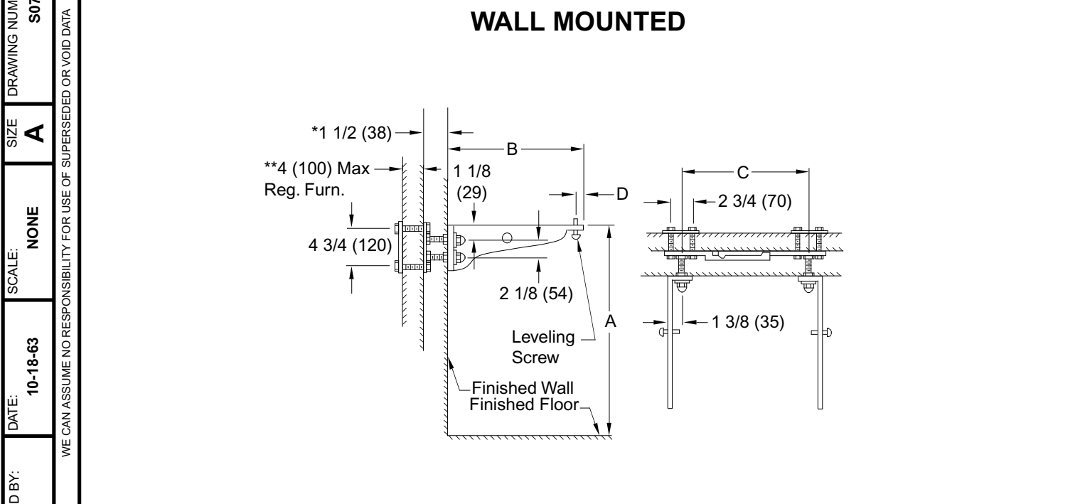
Fig. 0772 ... WITH OFFSET ACID RESISTANT COATED EXPOSED ARMS FOR HIGH BACK ENAMELED IRON LAVATORIES SET ON MASONRY OR STUD WALL
