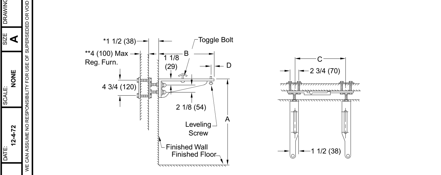
Fig. 0770 . . . WITH ACID RESISTANT COATED EXPOSED ARMS FOR FLAT SLAB AND HIGH BACK LAVATORIES SET ON MASONRY OR STUD WALL
