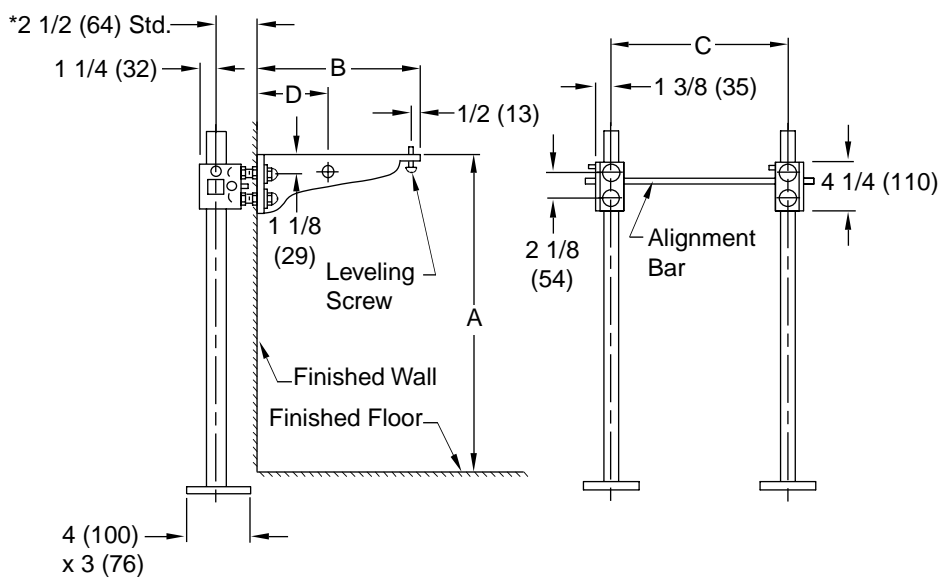
Fig. 0752 . . . WITH OFFSET ARMS FOR HIGH BACK ENAMELED IRON LAVATORIES
