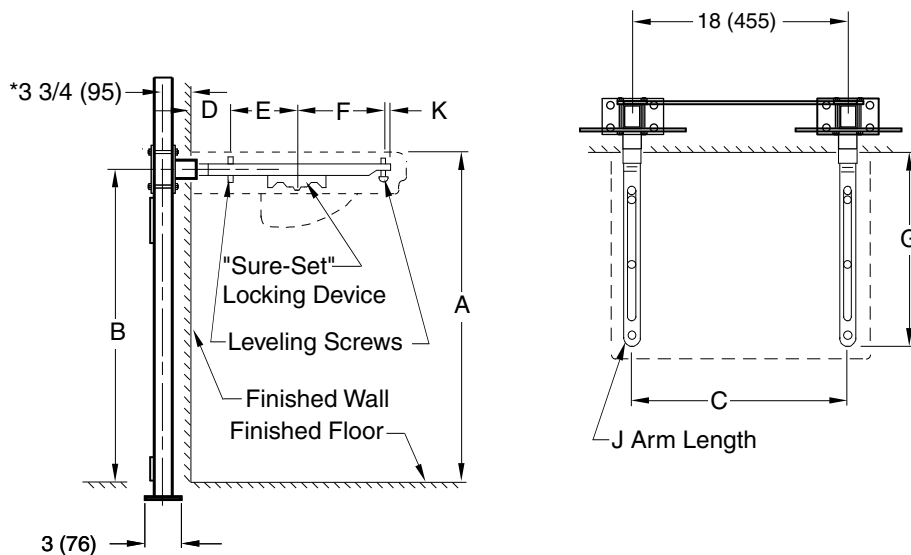
Fig. 0710 (-27) ... FOR HIGH BACK LAVATORIES (shown)
