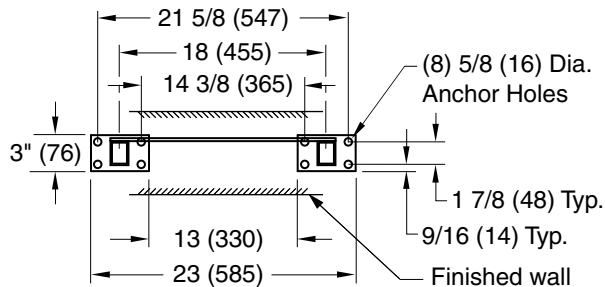
BASE DETAIL
