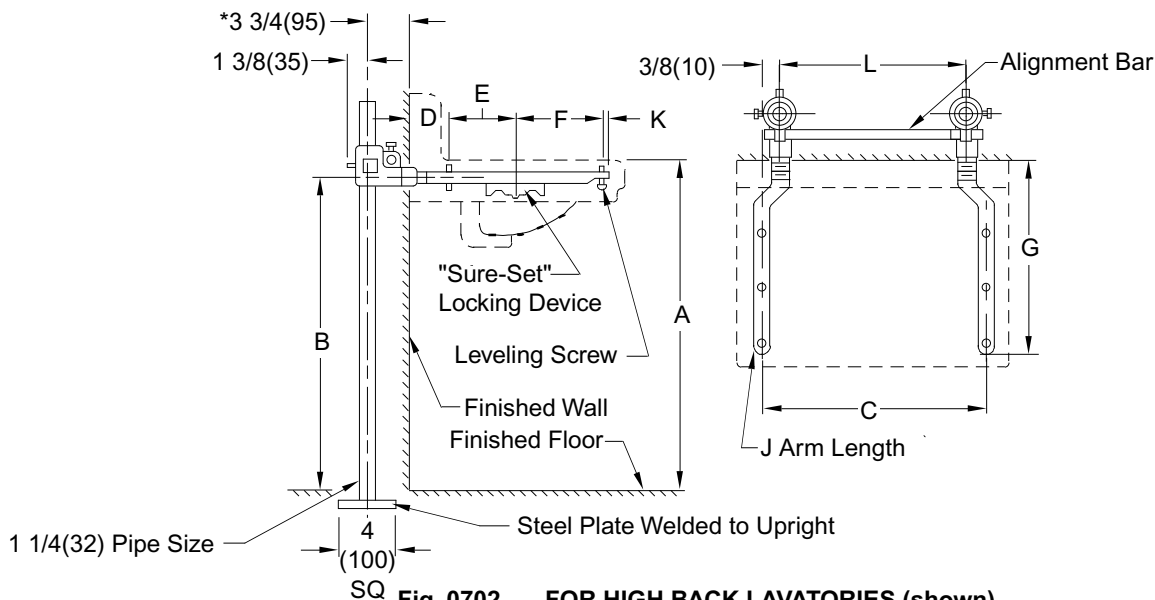
Fig. 0702 ... FOR HIGH BACK LAVATORIES (shown)
