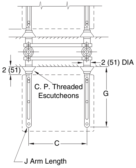
Fig. 0700D (-E) . . . FOR FLAT SLAB LAVATORIES (shown)
