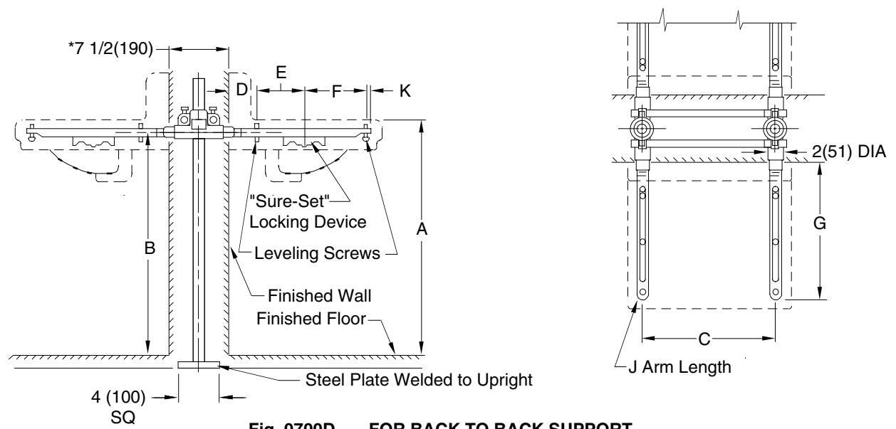
Fig. 0700D . . . FOR BACK TO BACK SUPPORT
