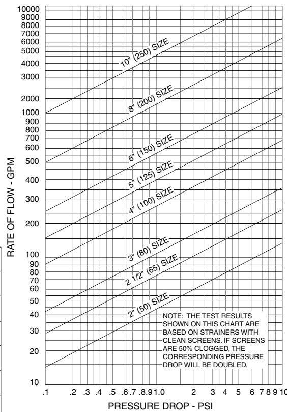
PRESSURE DROP THROUGH FIG. 8790 AND FIG. 8795 AT VARIABLE FLOW RATES
