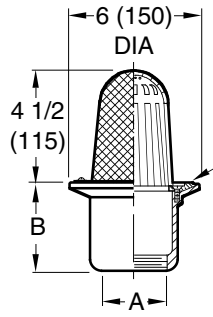
THREADED OUTLET Caulk When Specified
