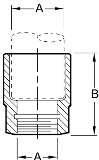
Fig. 2641T HUB ADAPTOR Female Thread Specify Type & Size eg: 2641T0125
