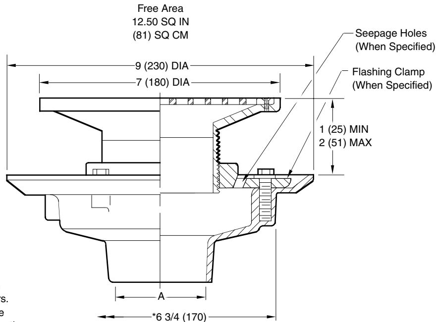
Fig. 2005Y (-SS) . . . NO-HUB OUTLET
