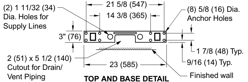
TOP AND BASE DETAIL
