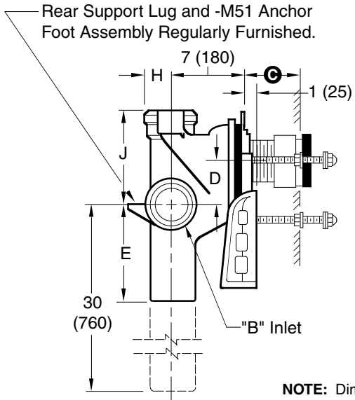
Fig. 0350 Side View
