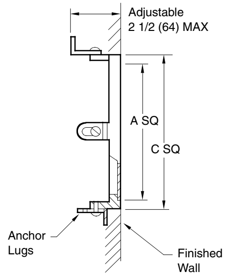
Fig. 4735 FLUSH-WITH-WALL COVER
