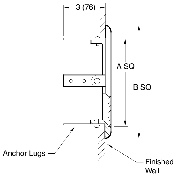
Fig. 4730 FACE-OF-WALL COVER
