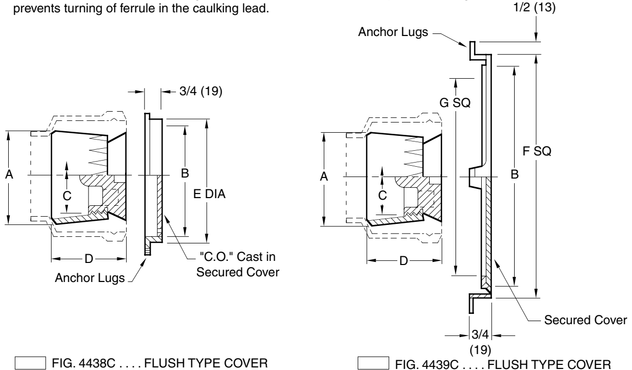
FIG. 4438C . . . . FLUSH TYPE COVER
