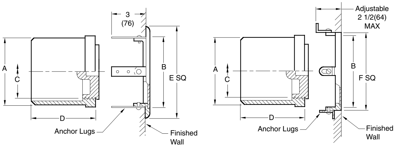
FIG. 4434C . . . . FACE-OF-WALL COVER
