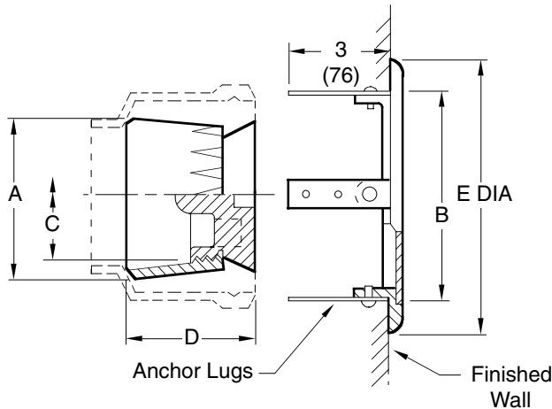
FIG. 4432C . . . . FACE-OF-WALL COVER
