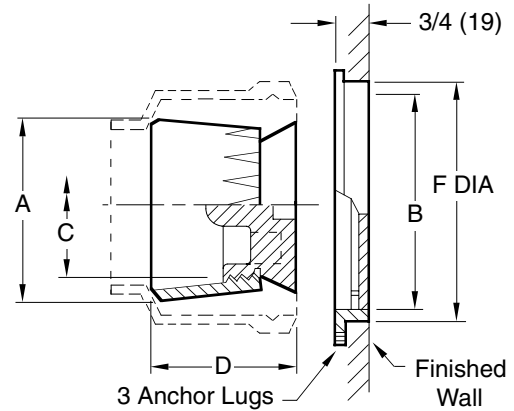
FIG. 4433C . . . . FLUSH-WITH-WALL COVER
