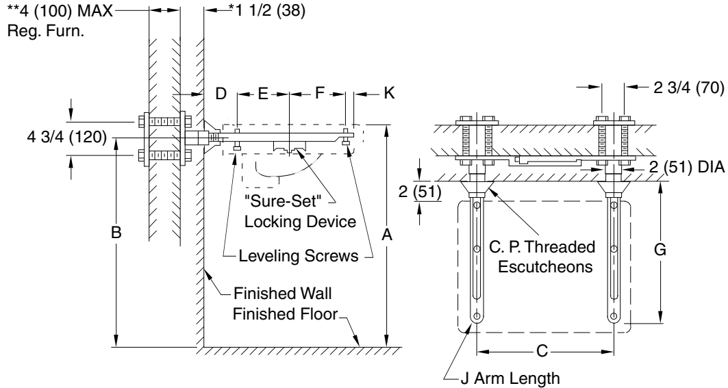
Fig. 0720 (-E) ... FOR FLAT SLAB LAVATORIES SET ON MASONRY OR STUD WALL
