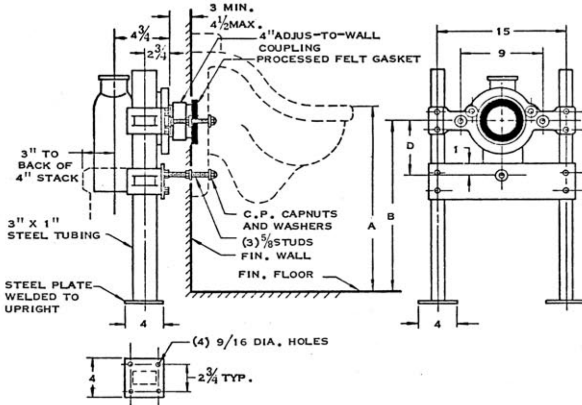
DETAIL OF HOLES IN BASE
