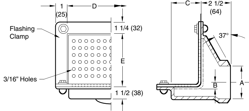
Fig. 9785FGSSBW... BUTT WELD OUTLET
