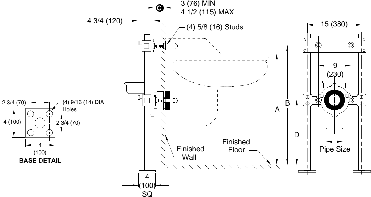
Fig. 0915 . . . WITH SUPPORTING STUDS, ADJUSTABLE COUPLING AND WASTE FITTING 4" (100) CAULK AND 4" (100) VENT FOR BACK OUTLET FLUSHING RIM SERVICE SINK
