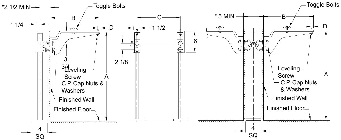
Fig. 0751... WITH ACID RESISTANT COATED EXPOSED ARMS FOR FLAT SLAB AND HIGH BACK LAVATORIES Fig. 0751D... WITH ACID RESISTANT COATED EXPOSED ARMS FOR FLAT SLAB AND HIGH BACK LAVATORIES
