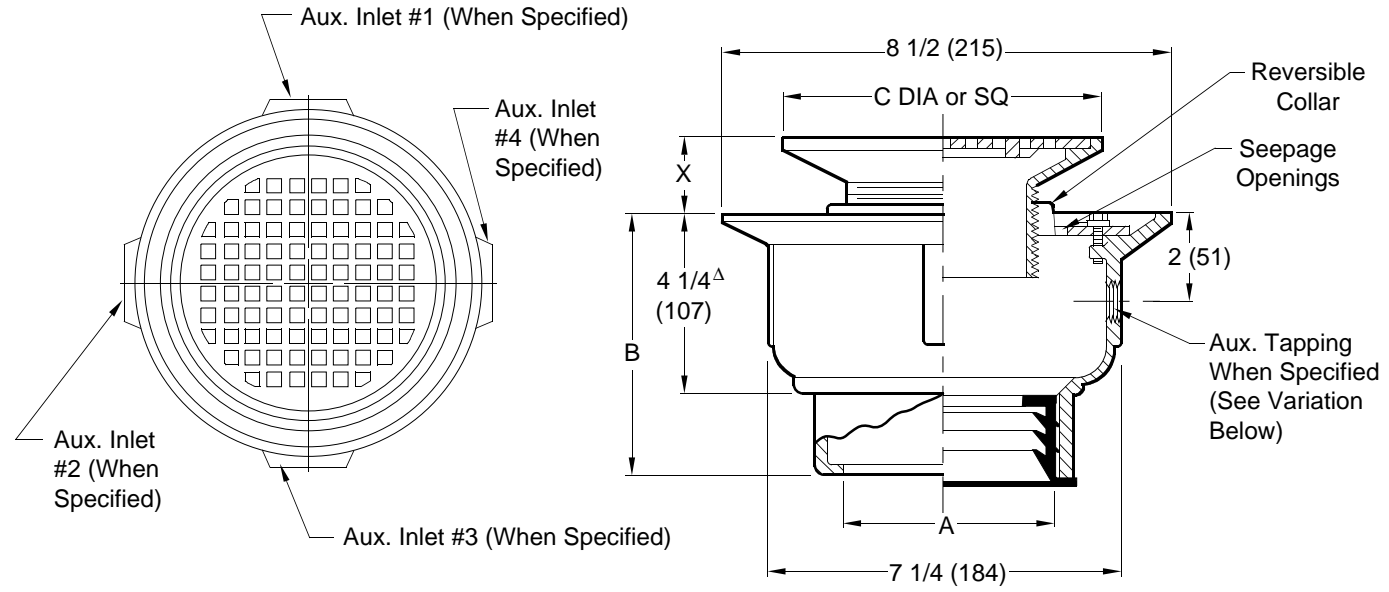
Fig. 2091Y . . . . . NO-HUB OUTLET (Regularly Furnished)
