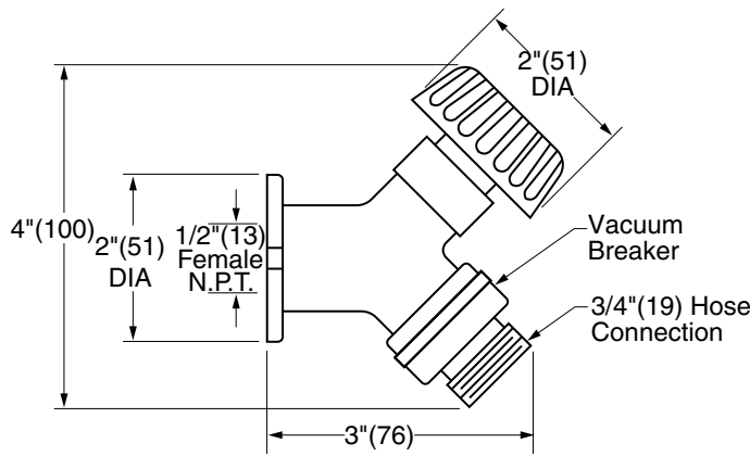
Fig. 5672.....1/2"(13) Inlet
